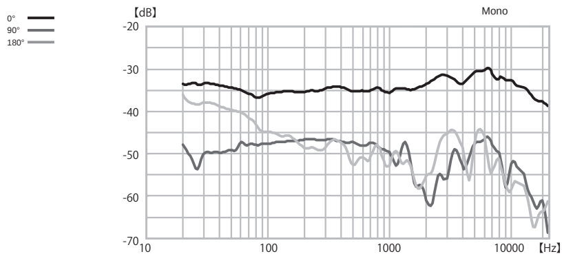
Frequency Response
