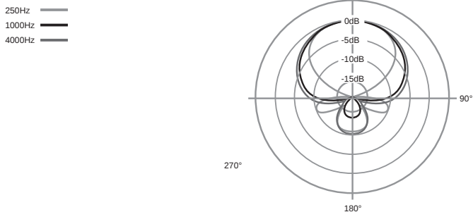
Polar Pattern
