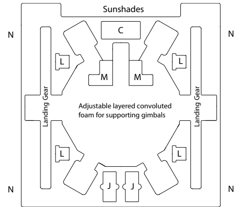
Bottom Tray
